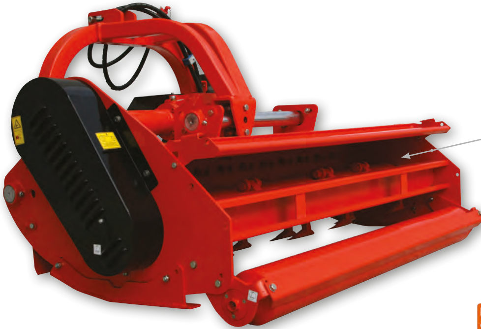
Double skinned deck
